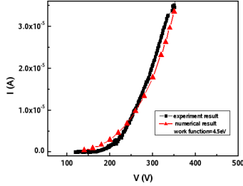
Fig. 6. Comparison of simulated and measured I-V curve.
