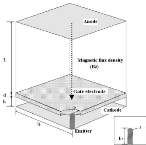
Fig. 3. Schematic diagram of the 1/4 simulation domain for a typical CNT-based triode-type field emitter within a periodic cell. Important geometrical parameters are: R=500\text{nm} , r=10\text{nm} , h_e=600\text{nm} , h=500\text{nm} , d=200\text{nm} , L=0.9\text{mm} and W=0.3\text{mm} .
