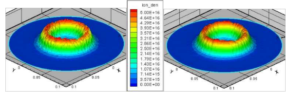
Fig. 8. Cycle-averaged distributions of number densities of electrons (left) and ions (right) for a RF magnetron argon plasma.
