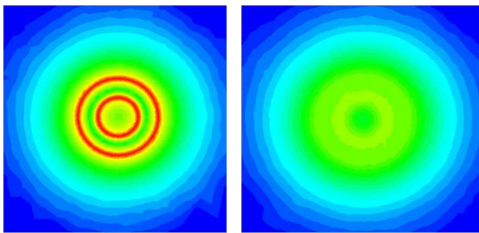
Fig. 7. Magnetic field strength at the mid-cross section of PM (left) and 0.002 m above the target electrode.
