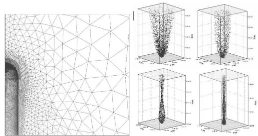
Fig. 4. From left to right, top to bottom: Exploded view of the refined mesh near the tip, instantaneous snapshot of electrons from a single-CNT triode-type field emitter with B=0, -0.2, -0.5, -1.0 Tesla. The gate voltage and the anode voltage are fixed at 120 Volts and 1 kV, respectively.
